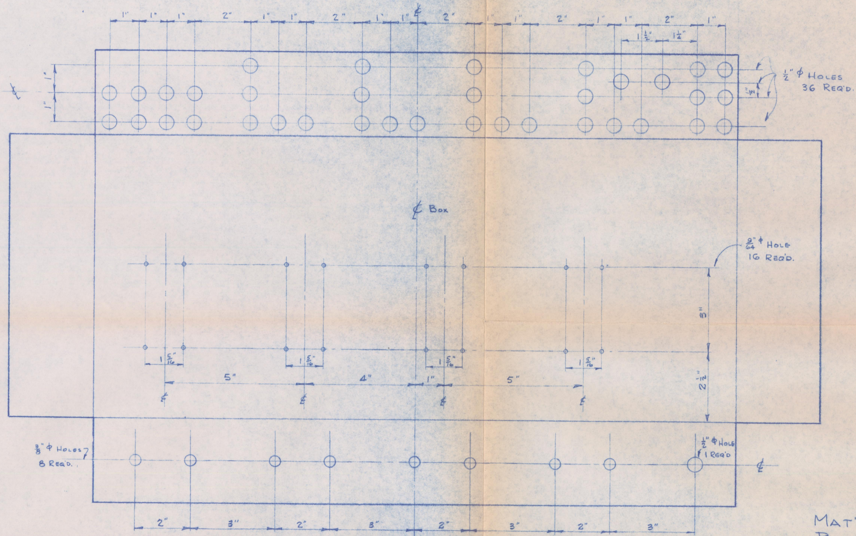
DEVELOPED VIEW
